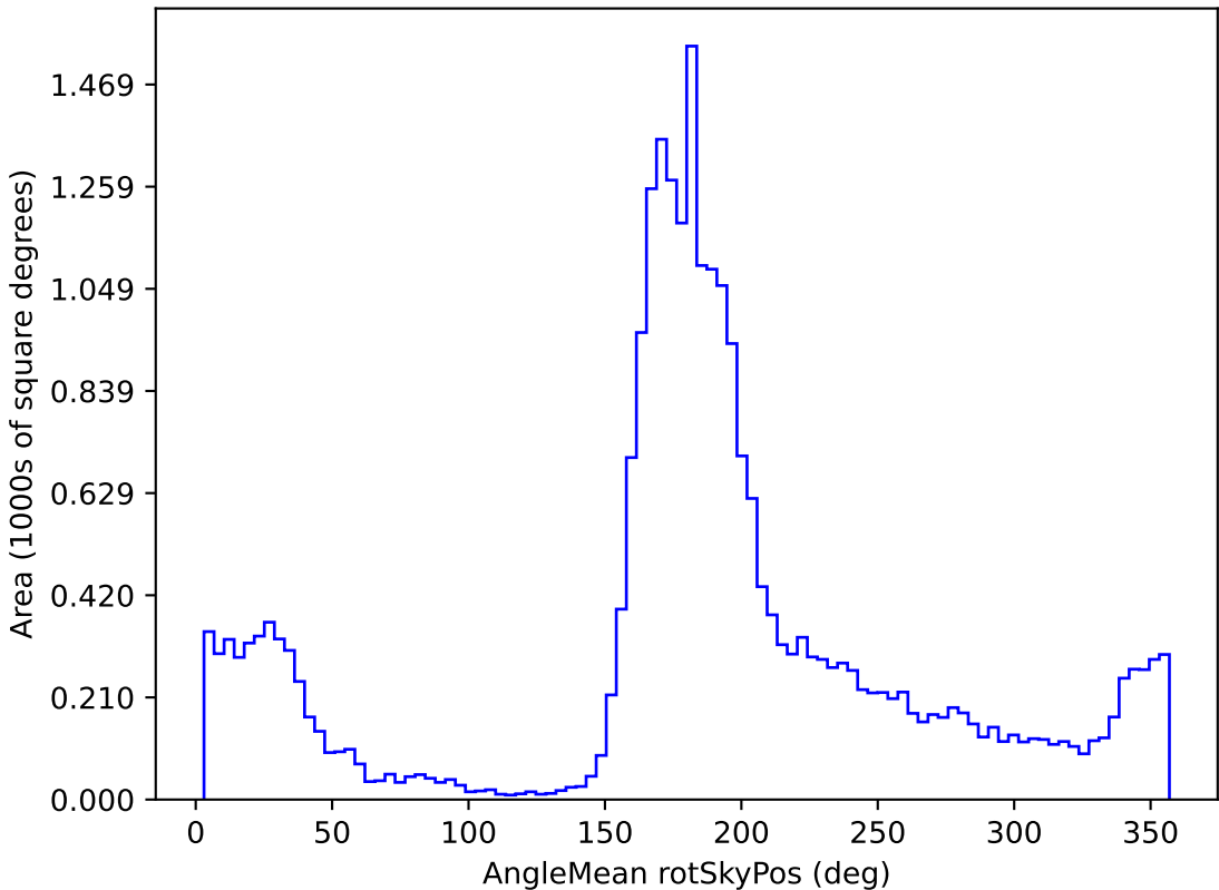
ddf_loaded_half_fl2_v3.4_10yrs All sky g band: AngleMean rotSkyPos
