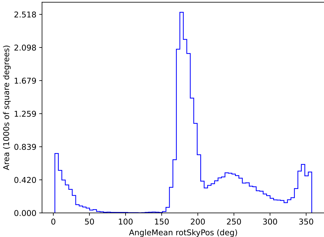
ddf_loaded_half_fl2_v3.4_10yrs All sky all bands: AngleMean rotSkyPos
