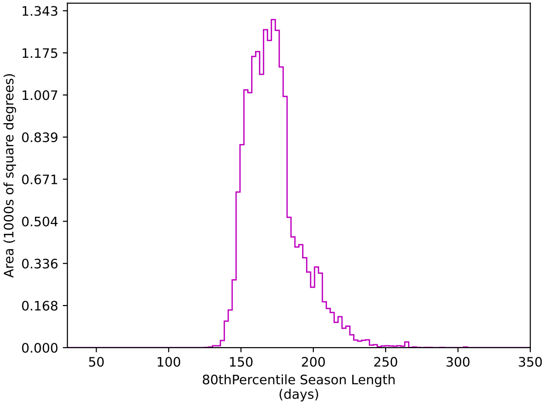
ddf_loaded_half_fl2_v3.4_10yrs WFD z band: 80thPercentile Season Length
