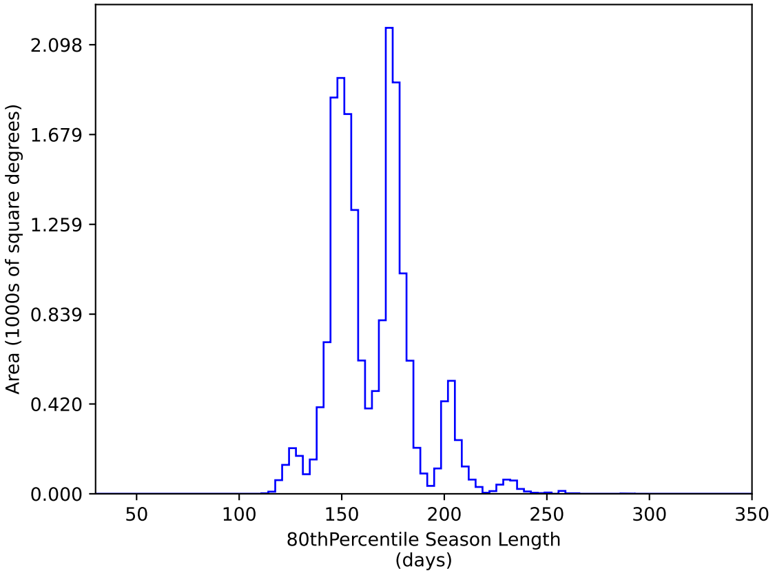
ddf_loaded_half_fl2_v3.4_10yrs WFD y band: 80thPercentile Season Length
