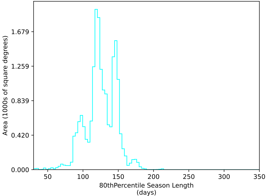
ddf_loaded_half_fl2_v3.4_10yrs WFD u band: 80thPercentile Season Length
