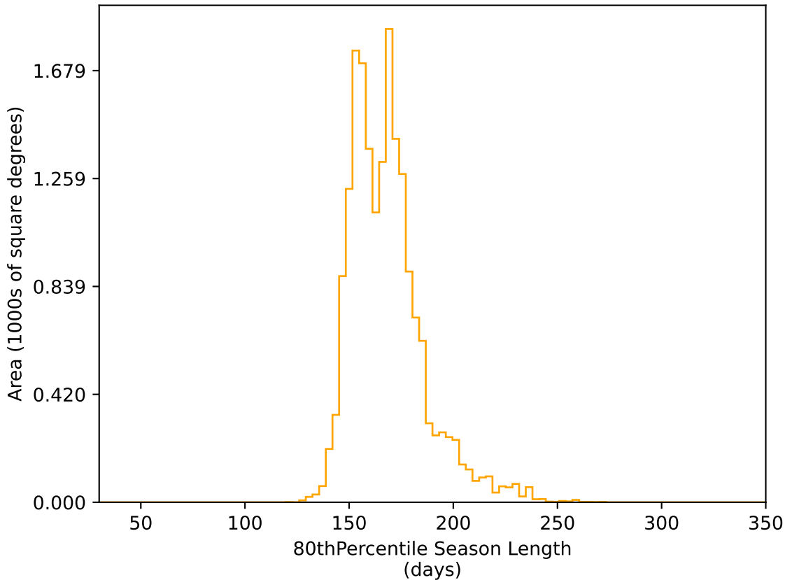
ddf_loaded_half_fl2_v3.4_10yrs WFD r band: 80thPercentile Season Length
