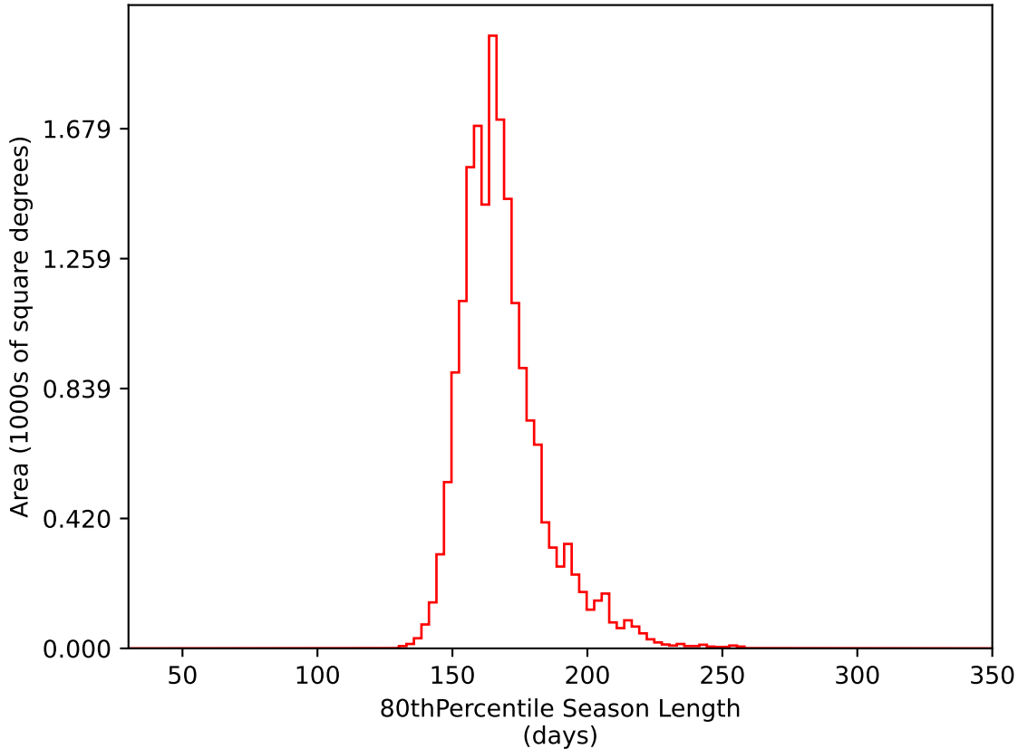
ddf_loaded_half_fl2_v3.4_10yrs WFD i band: 80thPercentile Season Length
