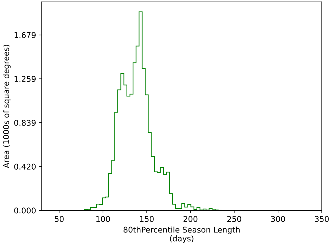
ddf_loaded_half_fl2_v3.4_10yrs WFD g band: 80thPercentile Season Length
