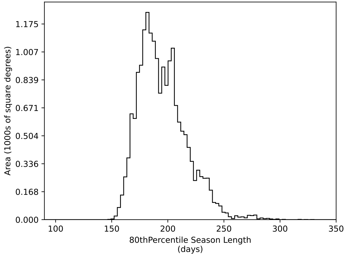
ddf_loaded_half_fl2_v3.4_10yrs WFD all bands: 80thPercentile Season Length
