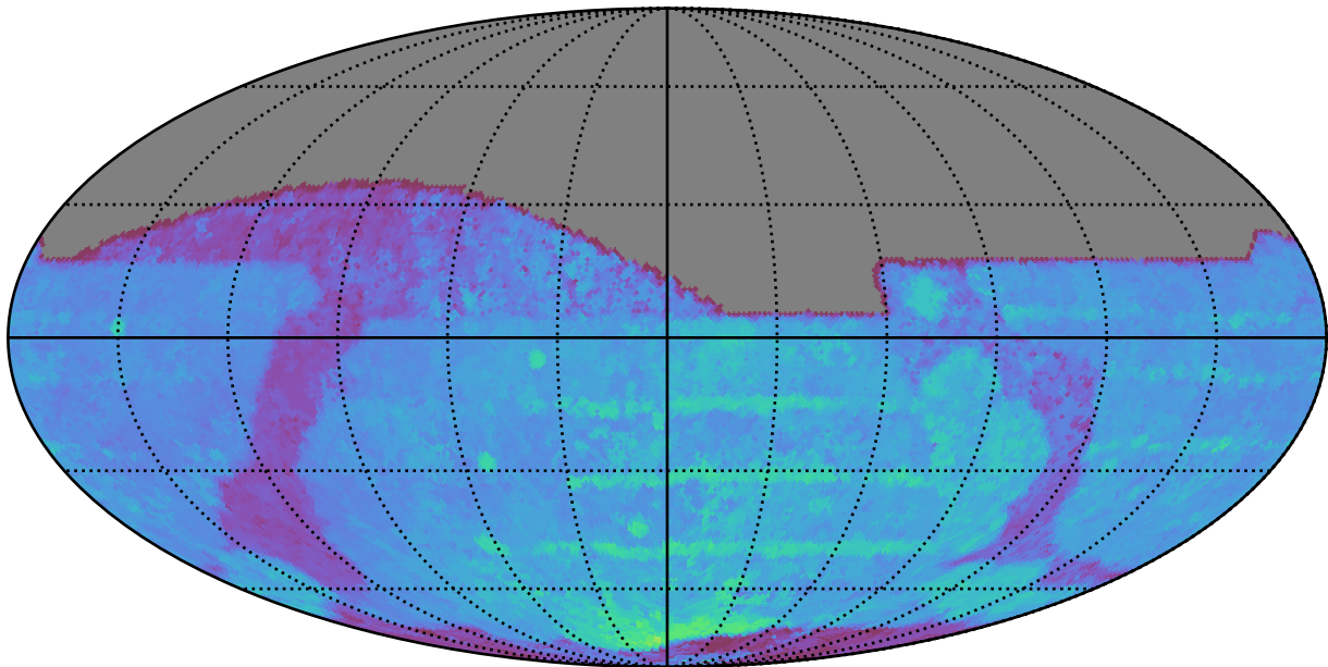
ddf_loaded_half_fl2_v3.4_10yrs All sky z band: 80thPercentile Season Length
