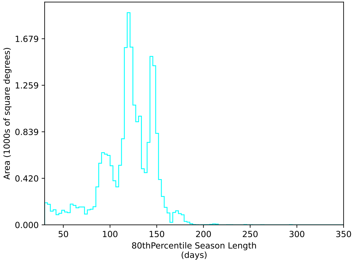
ddf_loaded_half_fl2_v3.4_10yrs All sky u band: 80thPercentile Season Length
