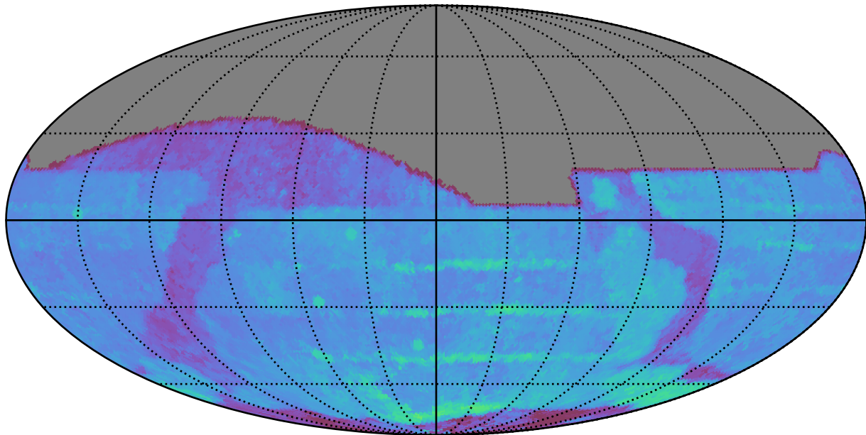
ddf_loaded_half_fl2_v3.4_10yrs All sky r band: 80thPercentile Season Length
