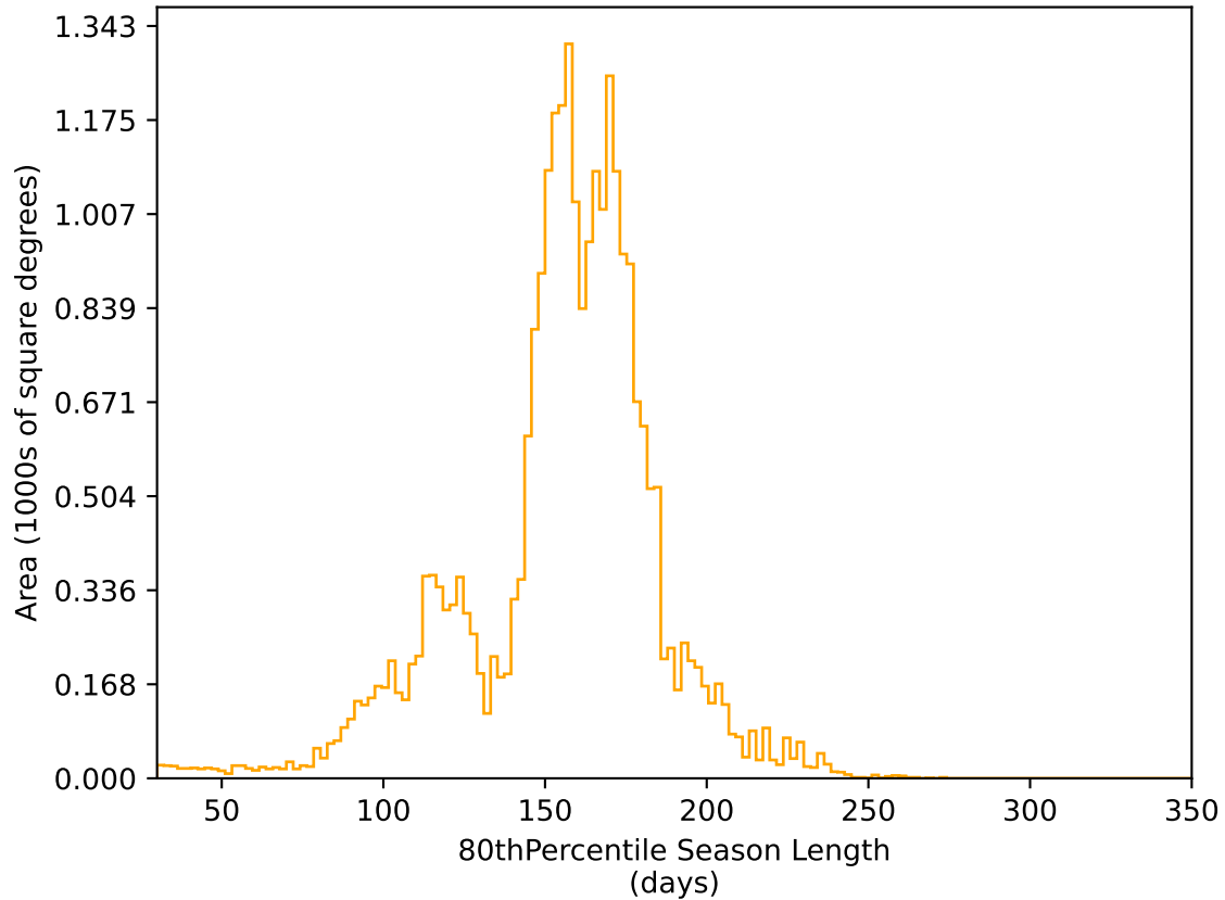
ddf_loaded_half_fl2_v3.4_10yrs All sky r band: 80thPercentile Season Length
