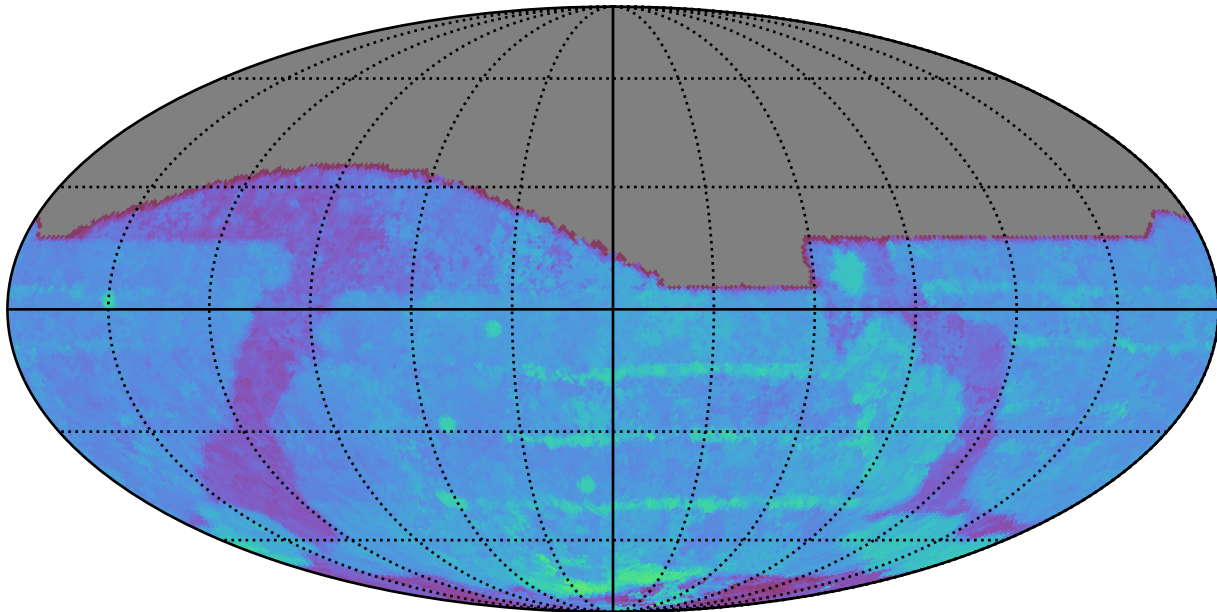
ddf_loaded_half_fl2_v3.4_10yrs All sky i band: 80thPercentile Season Length
