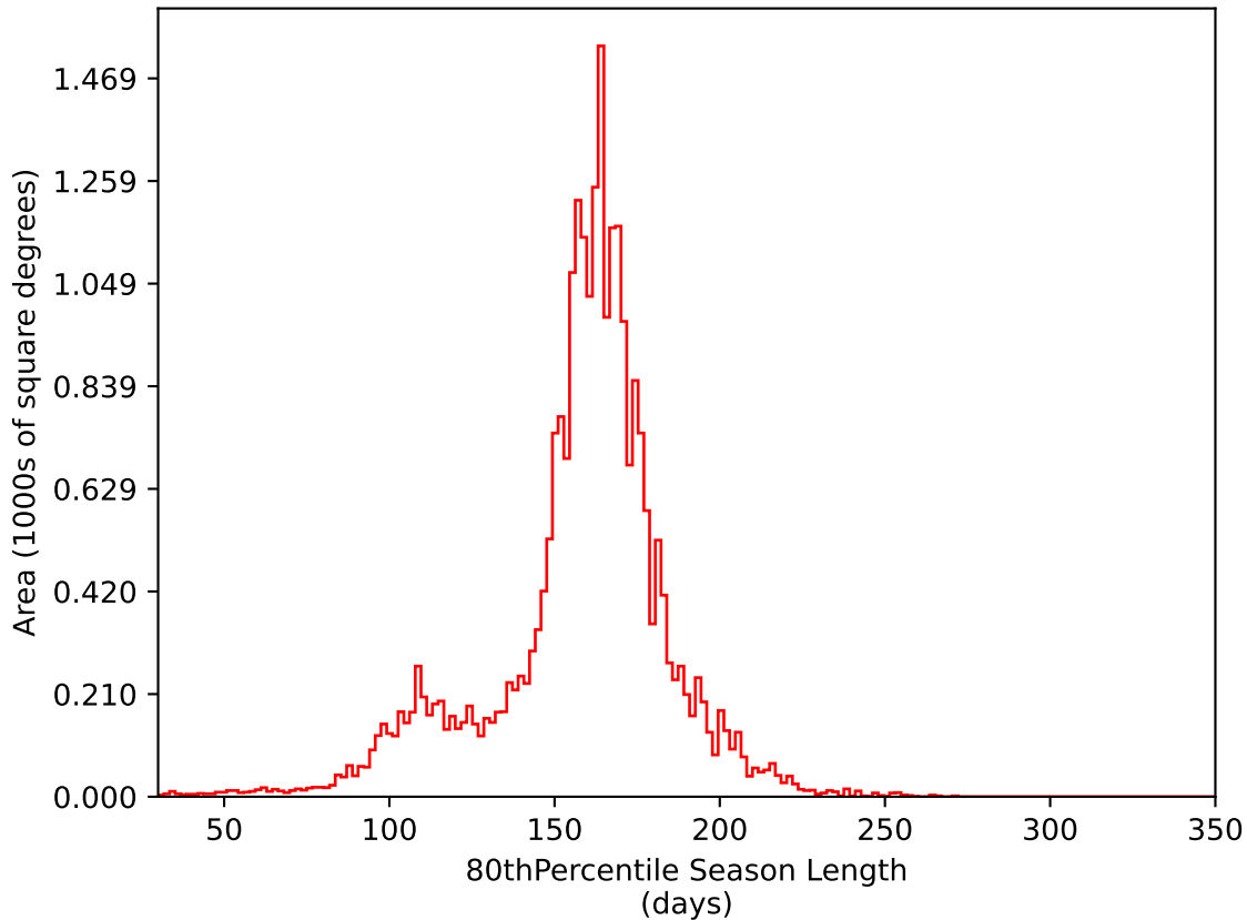
ddf_loaded_half_fl2_v3.4_10yrs All sky i band: 80thPercentile Season Length
