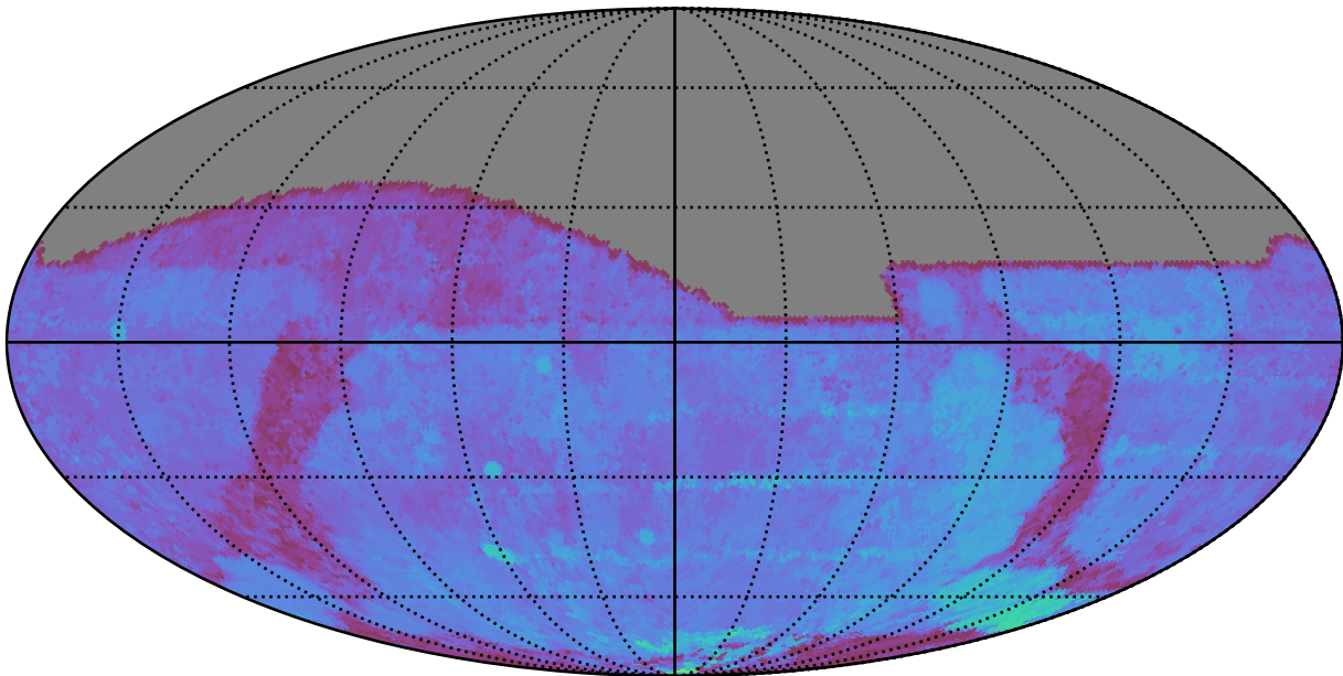
ddf_loaded_half_fl2_v3.4_10yrs All sky g band: 80thPercentile Season Length
