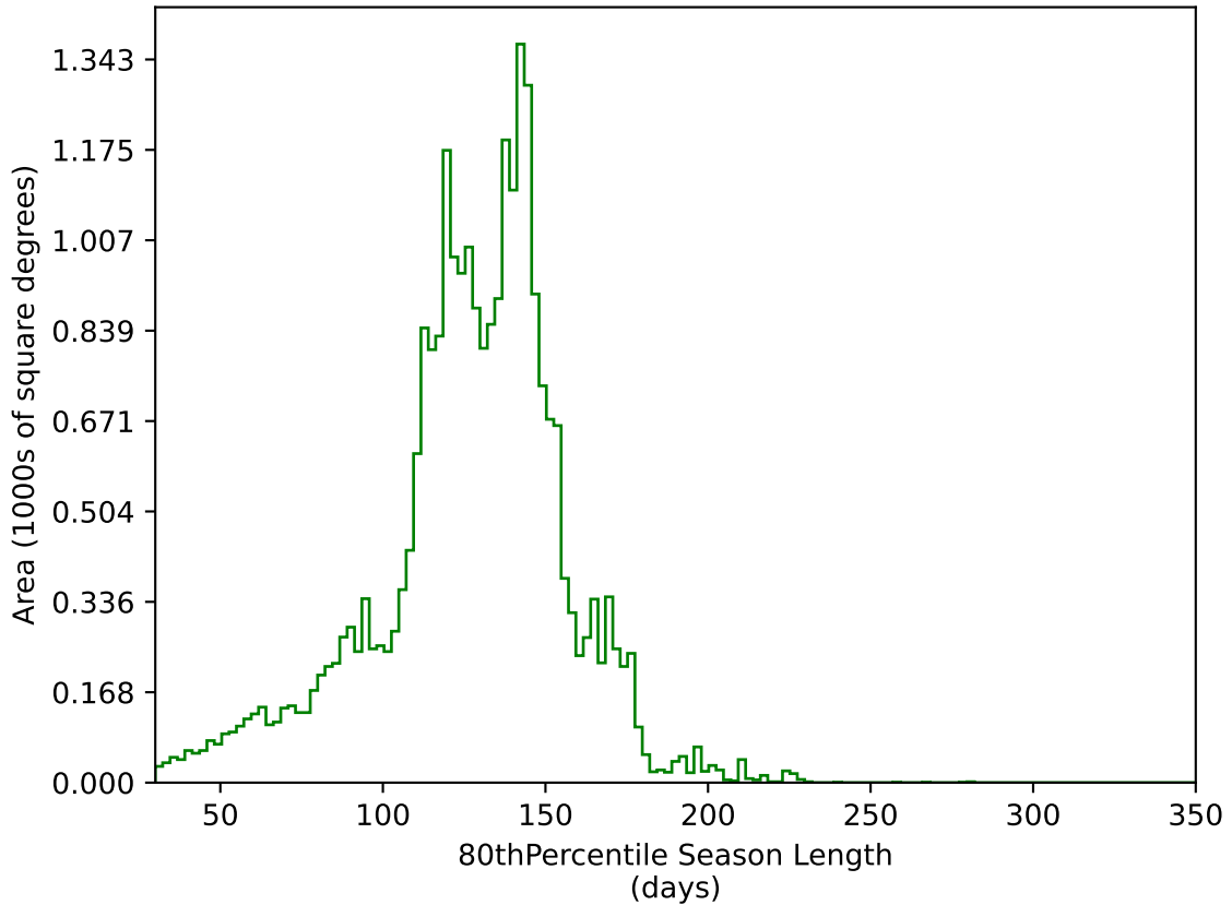
ddf_loaded_half_fl2_v3.4_10yrs All sky g band: 80thPercentile Season Length
