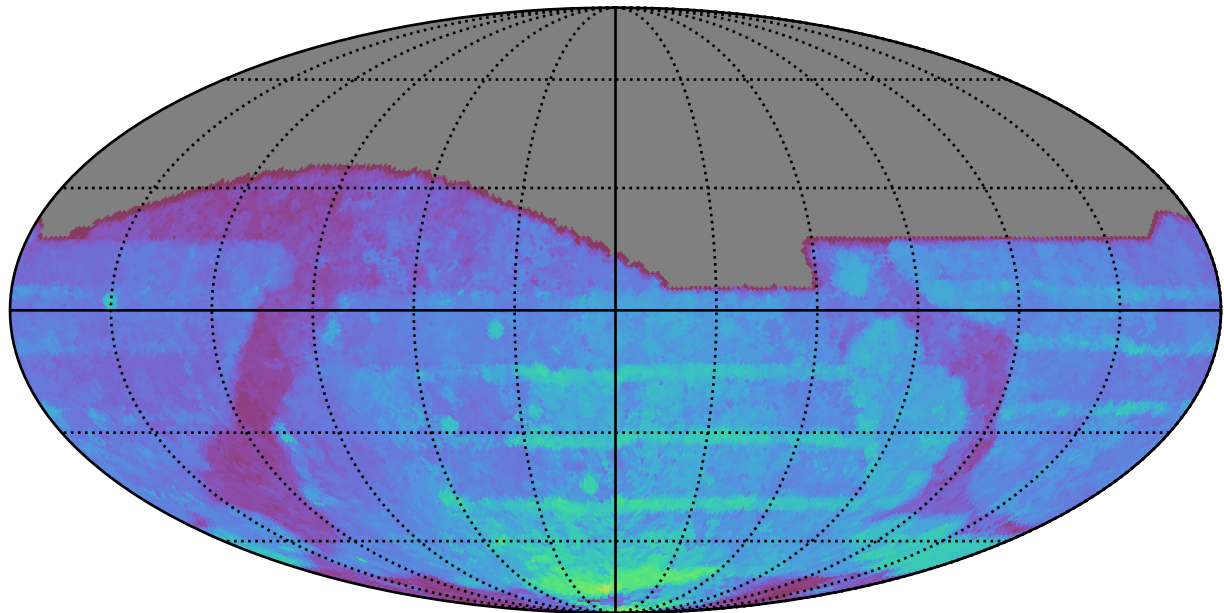
ddf_loaded_half_fl2_v3.4_10yrs All sky all bands: 80thPercentile Season Length
