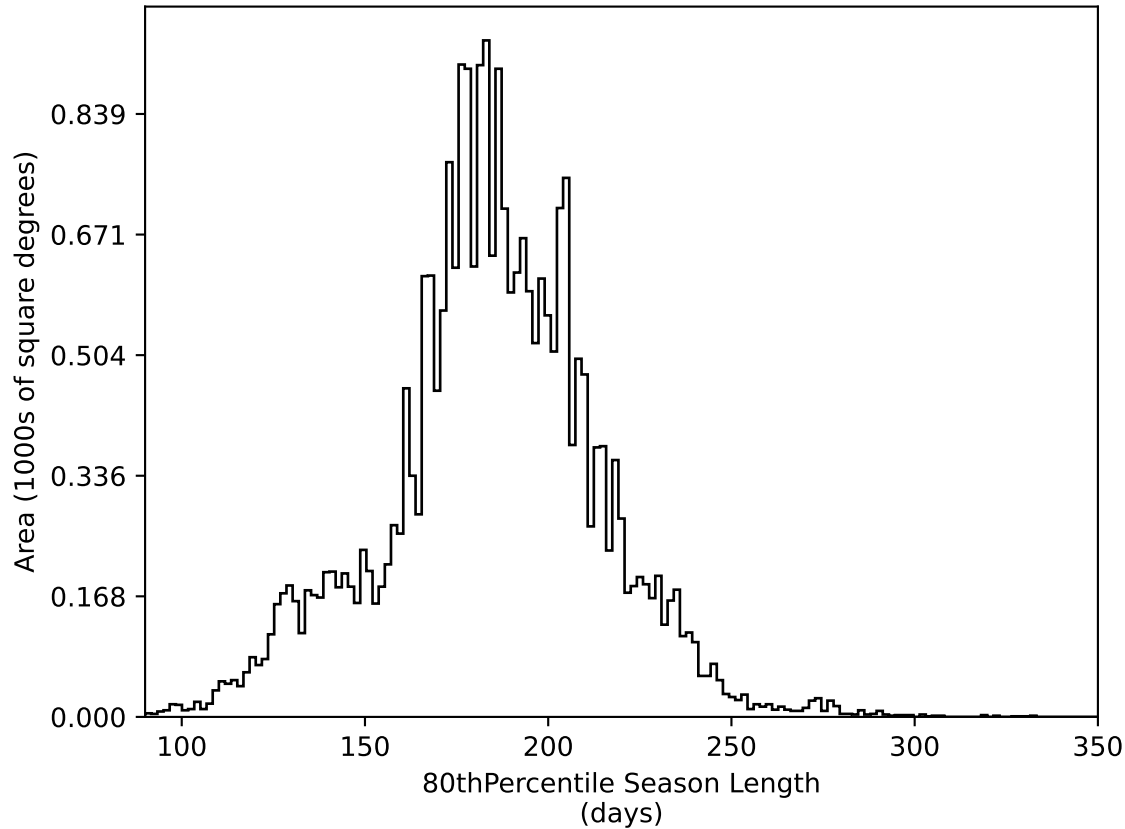
ddf_loaded_half_fl2_v3.4_10yrs All sky all bands: 80thPercentile Season Length
