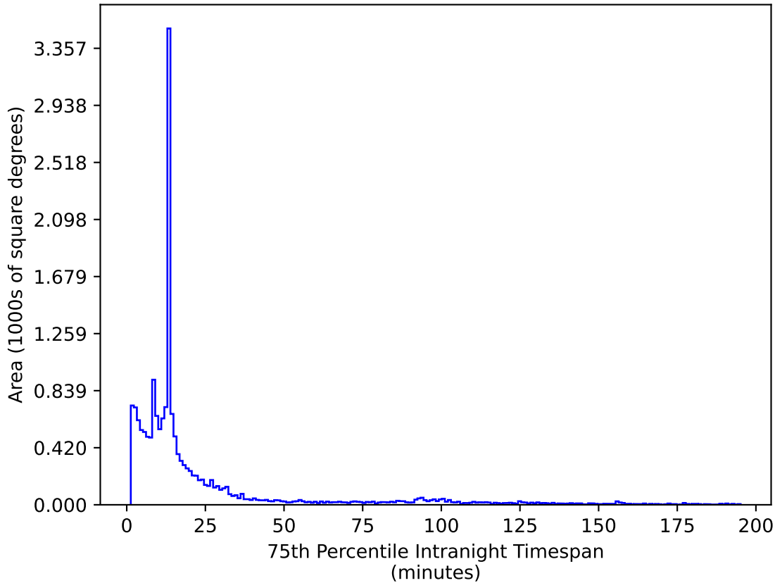
ddf_loaded_half_fl2_v3.4_10yrs WFD z band: 75th Percentile Intranight Timespan
