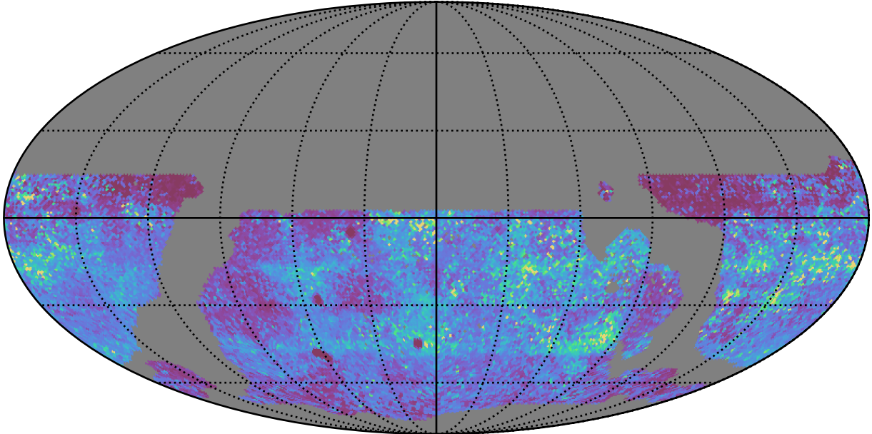
ddf_loaded_half_fl2_v3.4_10yrs WFD y band: 75th Percentile Intranight Timespan
