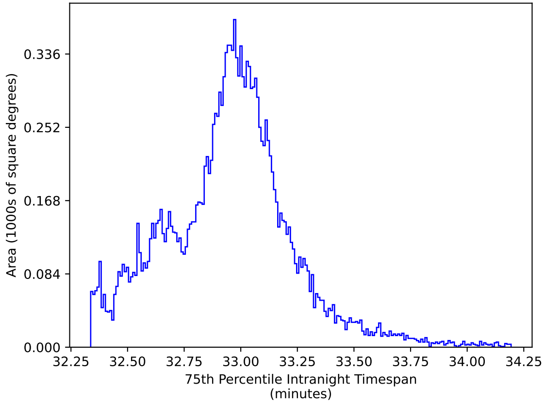
ddf_loaded_half_fl2_v3.4_10yrs WFD y band: 75th Percentile Intranight Timespan
