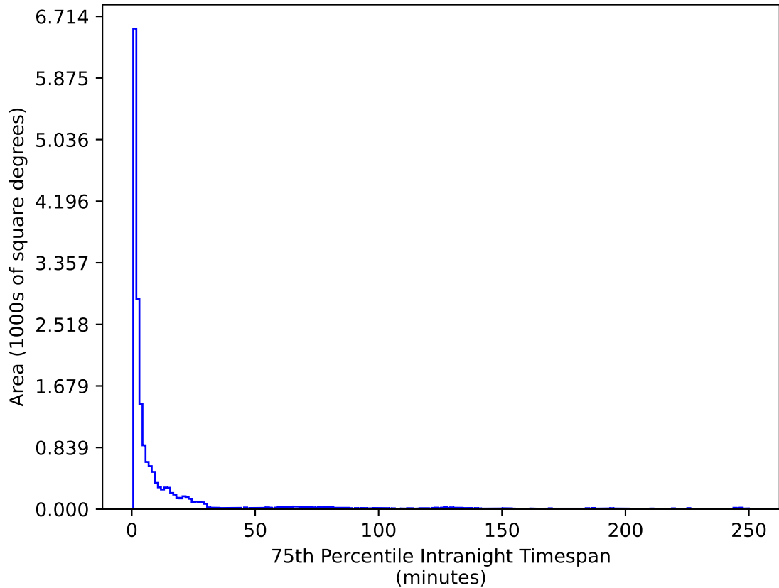
ddf_loaded_half_fl2_v3.4_10yrs WFD u band: 75th Percentile Intranight Timespan
