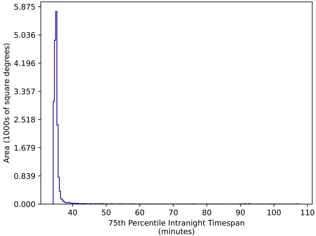
ddf_loaded_half_fl2_v3.4_10yrs WFD ri bands: 75th Percentile Intranight Timespan
