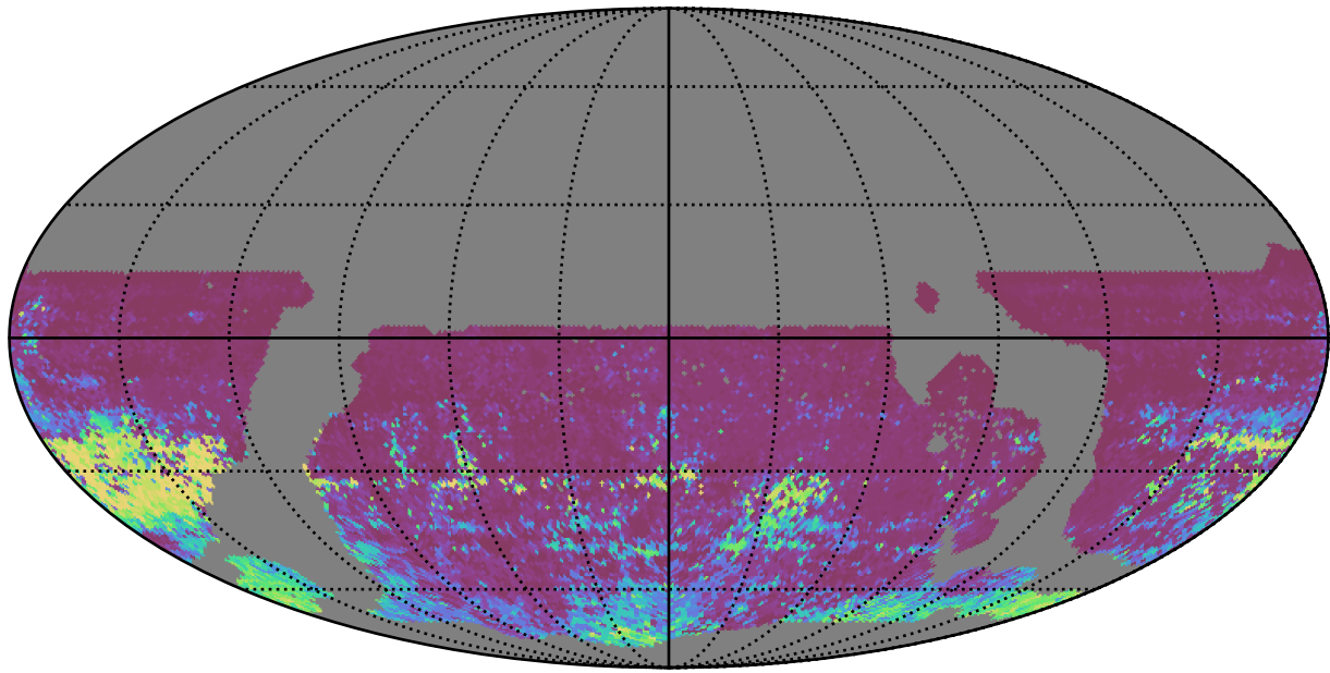
ddf_loaded_half_fl2_v3.4_10yrs WFD r band: 75th Percentile Intranight Timespan
