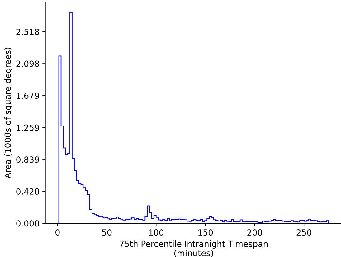
ddf_loaded_half_fl2_v3.4_10yrs WFD r band: 75th Percentile Intranight Timespan
