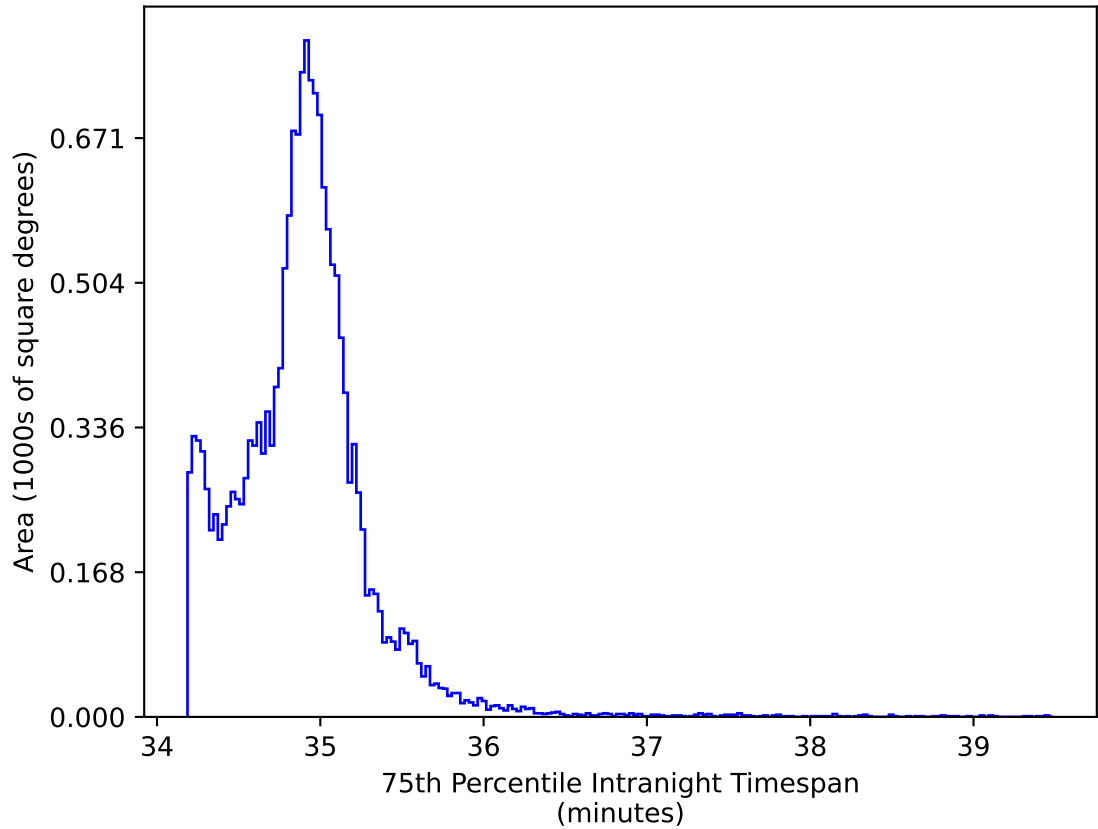
ddf_loaded_half_fl2_v3.4_10yrs WFD iz bands: 75th Percentile Intranight Timespan
