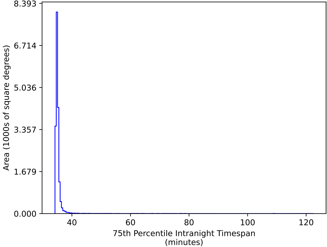
ddf_loaded_half_fl2_v3.4_10yrs WFD gr bands: 75th Percentile Intranight Timespan
