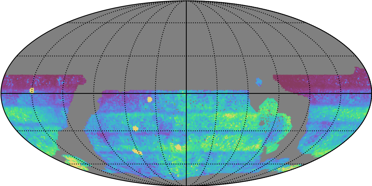
ddf_loaded_half_fl2_v3.4_10yrs WFD all bands: 75th Percentile Intranight Timespan
