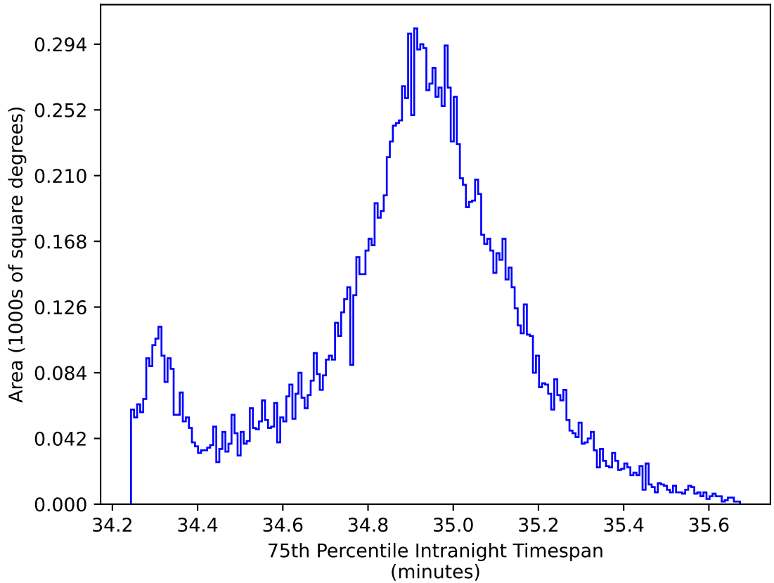
ddf_loaded_half_fl2_v3.4_10yrs WFD all bands: 75th Percentile Intranight Timespan
