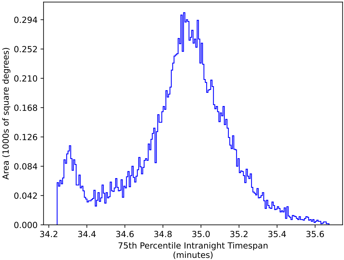
ddf_loaded_half_fl2_v3.4_10yrs WFD: 75th Percentile Intranight Timespan
