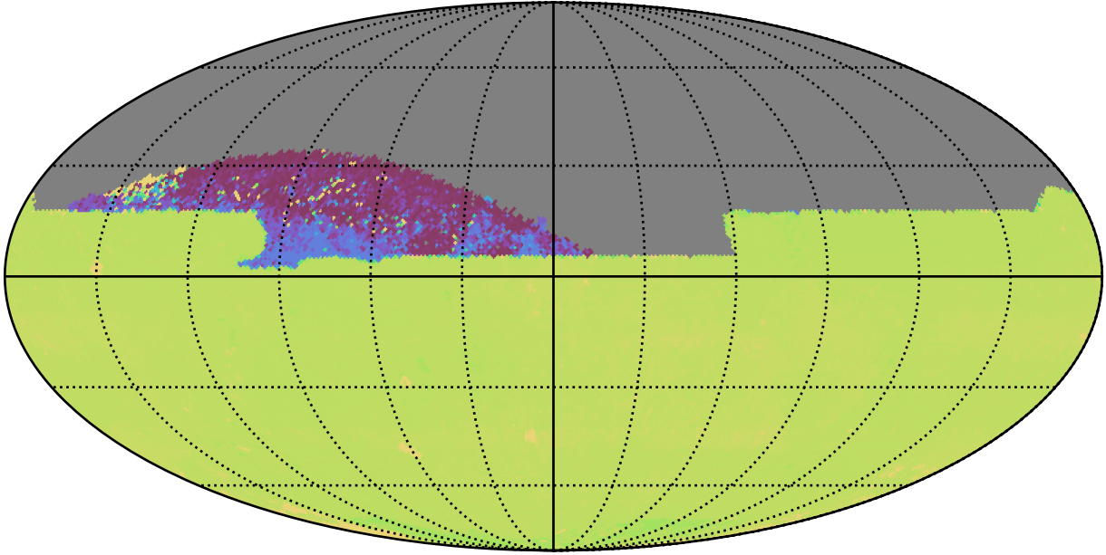
ddf_loaded_half_fl2_v3.4_10yrs All sky zy bands: 75th Percentile Intranight Timespan
