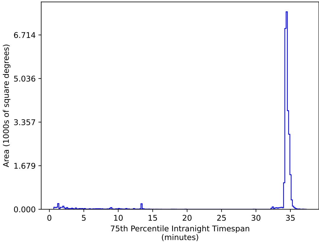
ddf_loaded_half_fl2_v3.4_10yrs All sky zy bands: 75th Percentile Intranight Timespan
