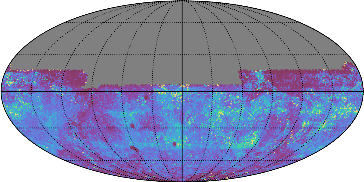
ddf_loaded_half_fl2_v3.4_10yrs All sky y band: 75th Percentile Intranight Timespan
