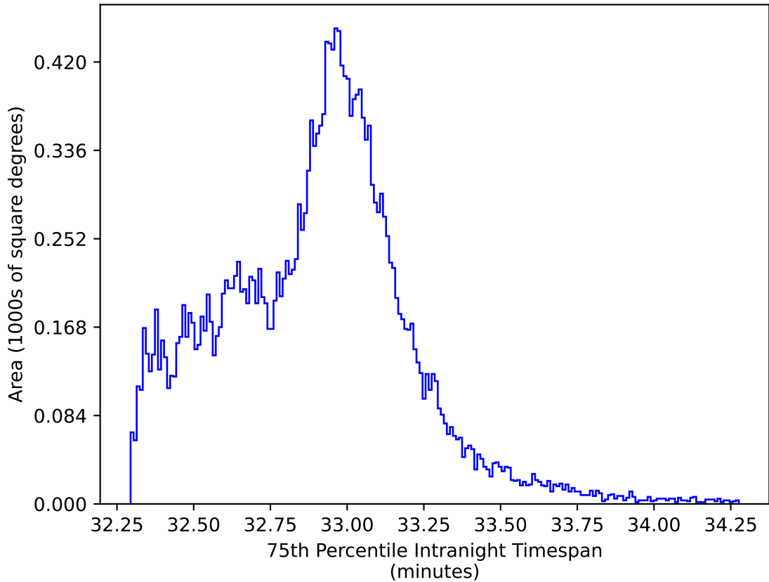
ddf_loaded_half_fl2_v3.4_10yrs All sky y band: 75th Percentile Intranight Timespan
