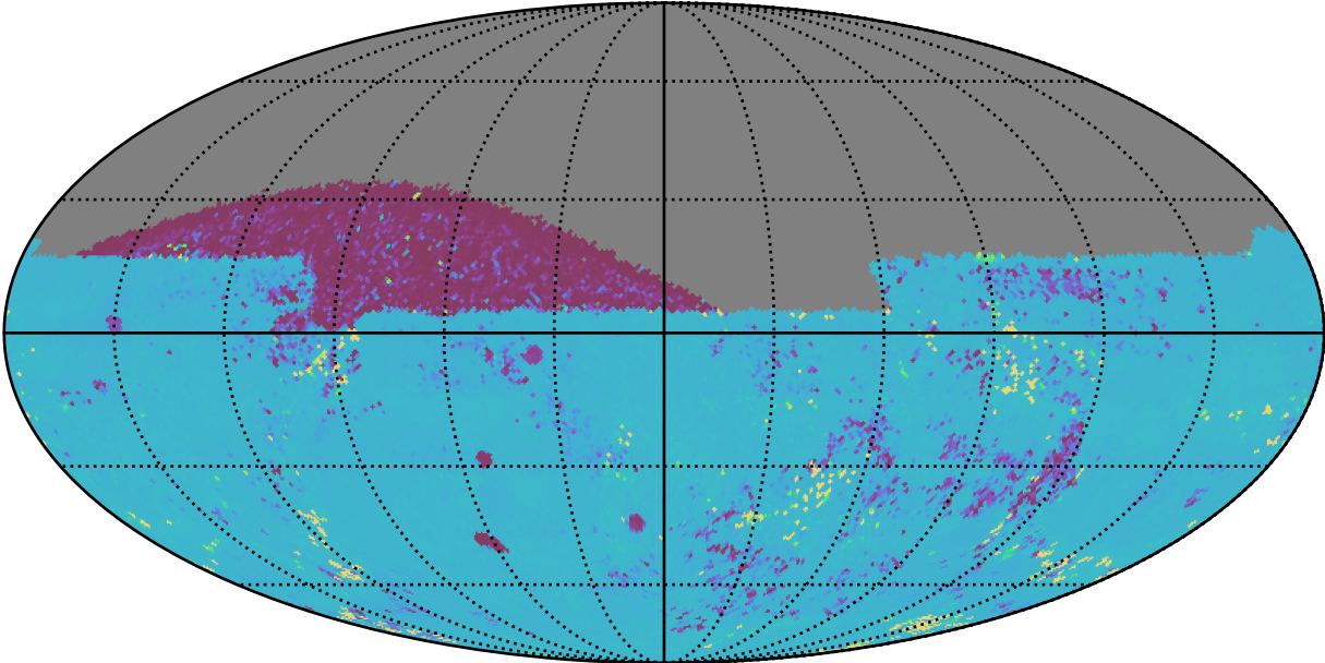
ddf_loaded_half_fl2_v3.4_10yrs All sky ug bands: 75th Percentile Intranight Timespan
