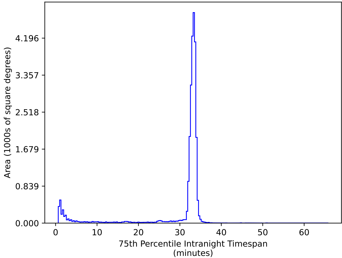
ddf_loaded_half_fl2_v3.4_10yrs All sky ug bands: 75th Percentile Intranight Timespan
