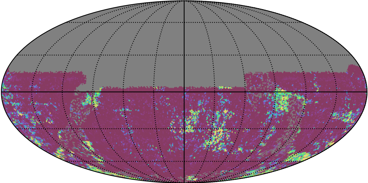
ddf_loaded_half_fl2_v3.4_10yrs All sky u band: 75th Percentile Intranight Timespan
