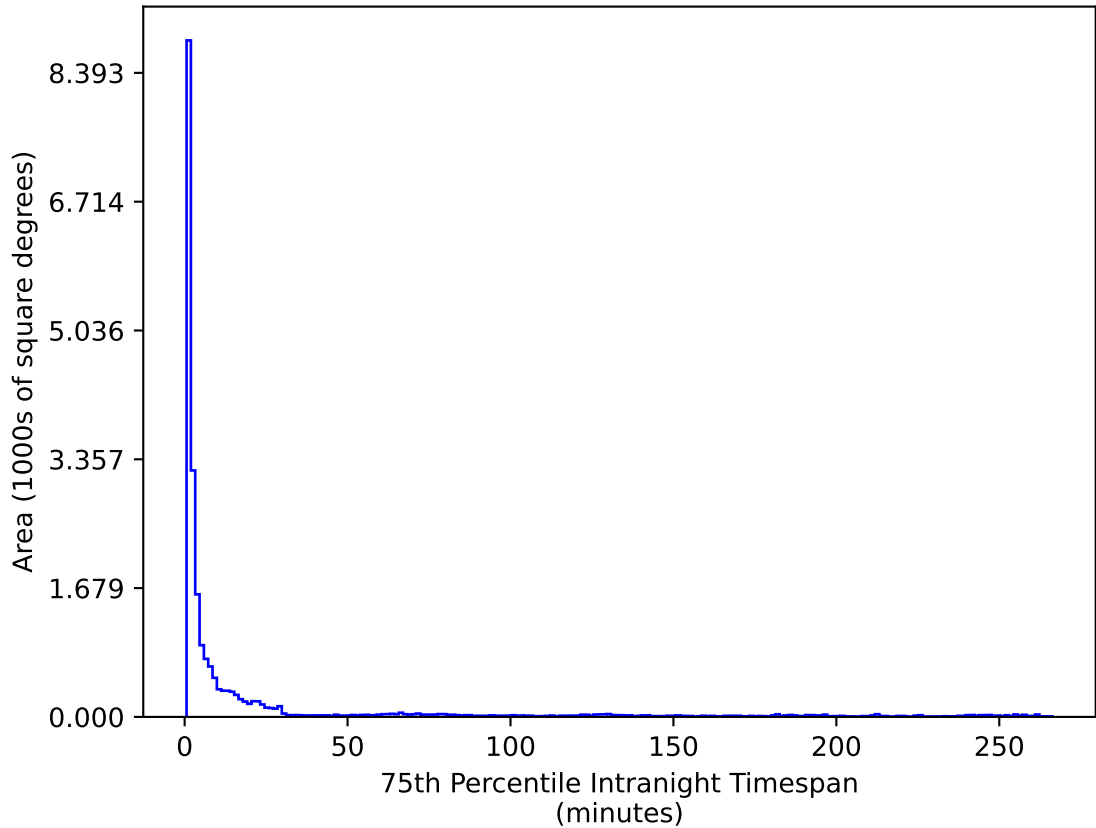
ddf_loaded_half_fl2_v3.4_10yrs All sky u band: 75th Percentile Intranight Timespan
