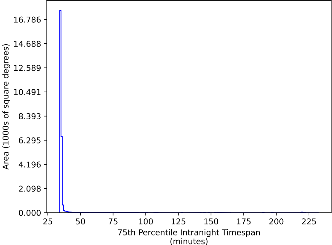
ddf_loaded_half_fl2_v3.4_10yrs All sky ri bands: 75th Percentile Intranight Timespan
