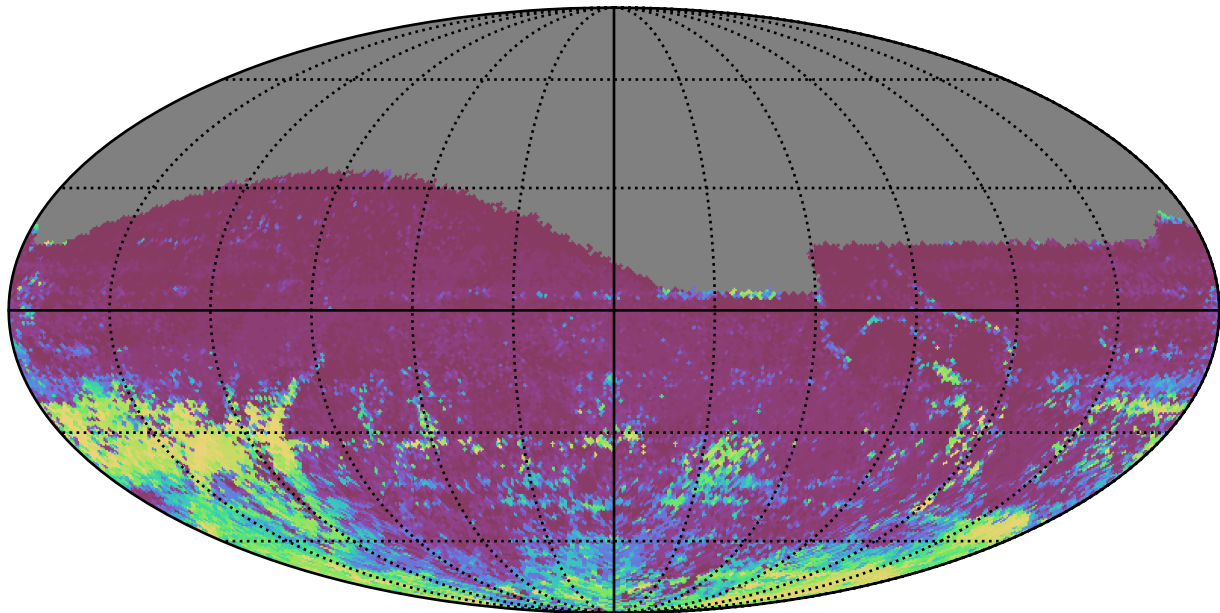
ddf_loaded_half_fl2_v3.4_10yrs All sky r band: 75th Percentile Intranight Timespan
