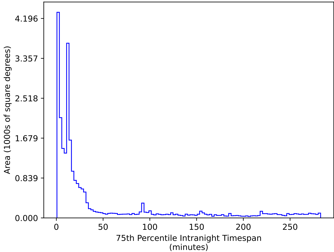
ddf_loaded_half_fl2_v3.4_10yrs All sky r band: 75th Percentile Intranight Timespan
