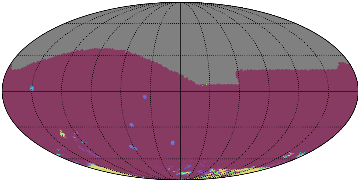
ddf_loaded_half_fl2_v3.4_10yrs All sky iz bands: 75th Percentile Intranight Timespan
