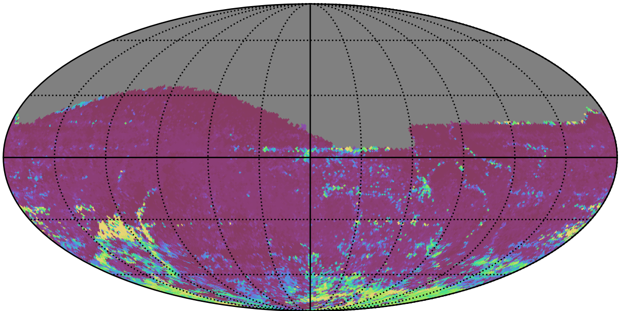
ddf_loaded_half_fl2_v3.4_10yrs All sky i band: 75th Percentile Intranight Timespan
