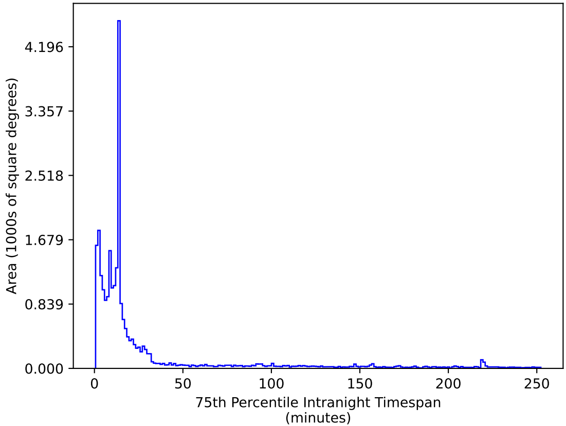
ddf_loaded_half_fl2_v3.4_10yrs All sky i band: 75th Percentile Intranight Timespan
