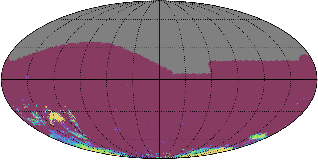
ddf_loaded_half_fl2_v3.4_10yrs All sky gr bands: 75th Percentile Intranight Timespan
