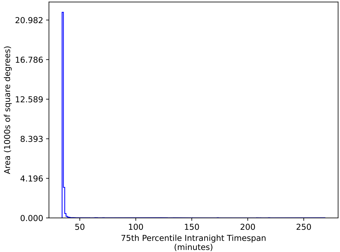
ddf_loaded_half_fl2_v3.4_10yrs All sky gr bands: 75th Percentile Intranight Timespan
