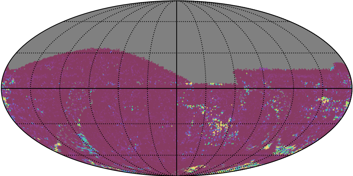
ddf_loaded_half_fl2_v3.4_10yrs All sky g band: 75th Percentile Intranight Timespan
