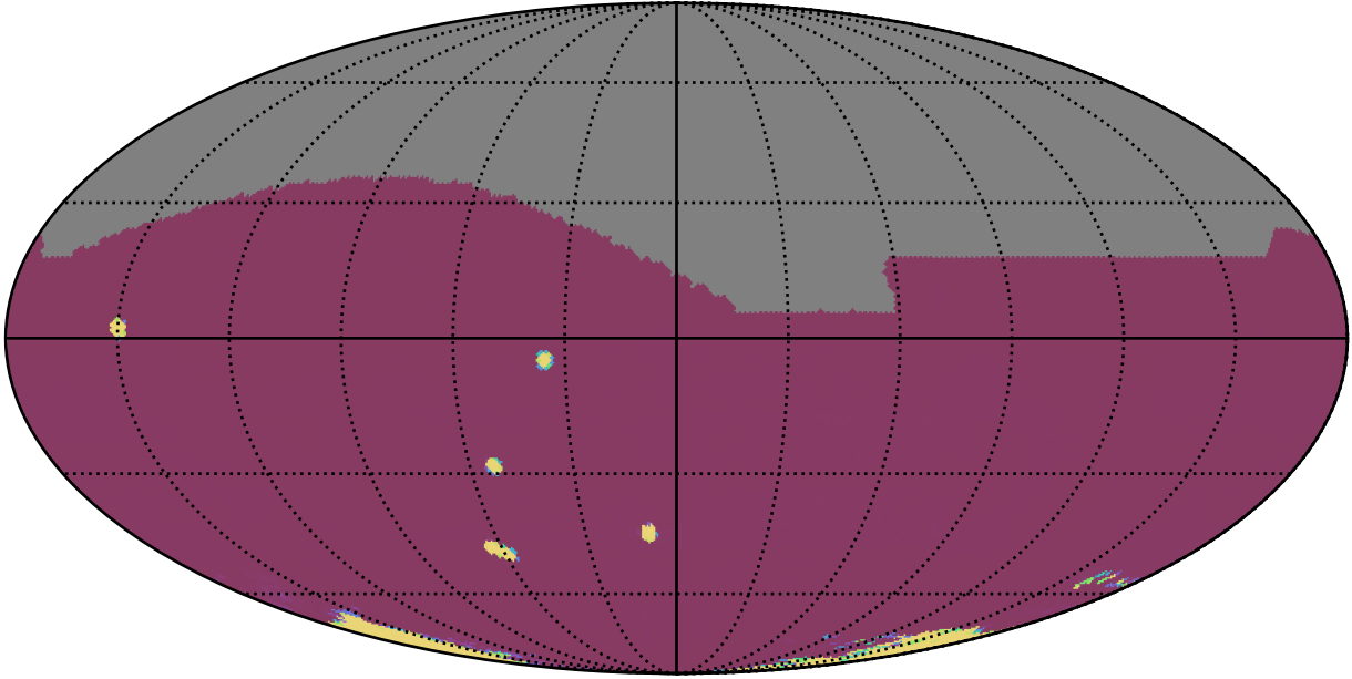
ddf_loaded_half_fl2_v3.4_10yrs All sky all bands: 75th Percentile Intranight Timespan
