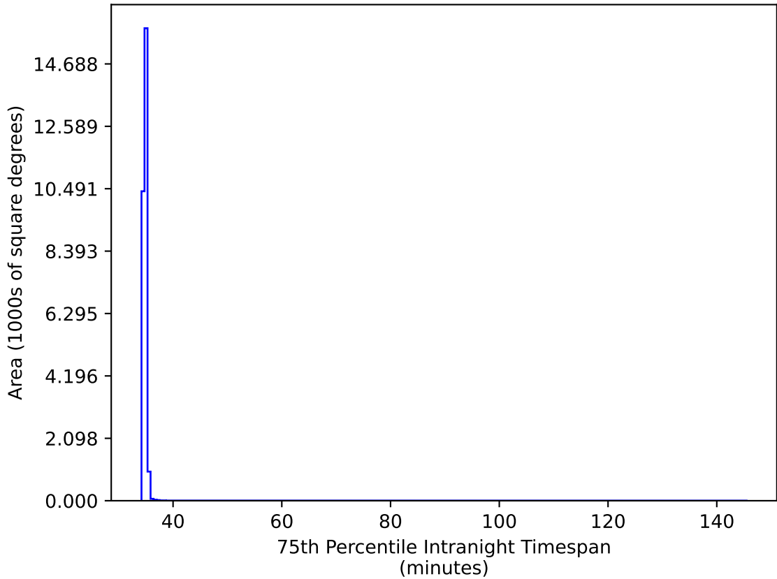
ddf_loaded_half_fl2_v3.4_10yrs All sky all bands: 75th Percentile Intranight Timespan
